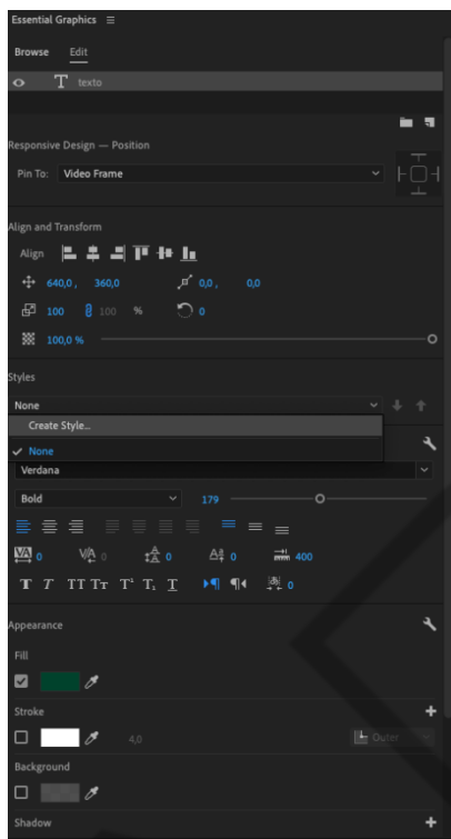
Figura 20 – Create style
